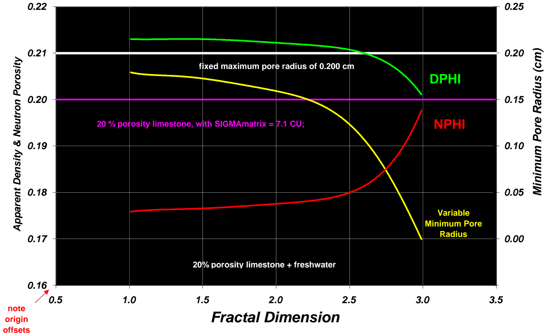
Density & Neutron Apparent Porosity versus Fractal Dimension with a Constant True Porosity of 0.20
