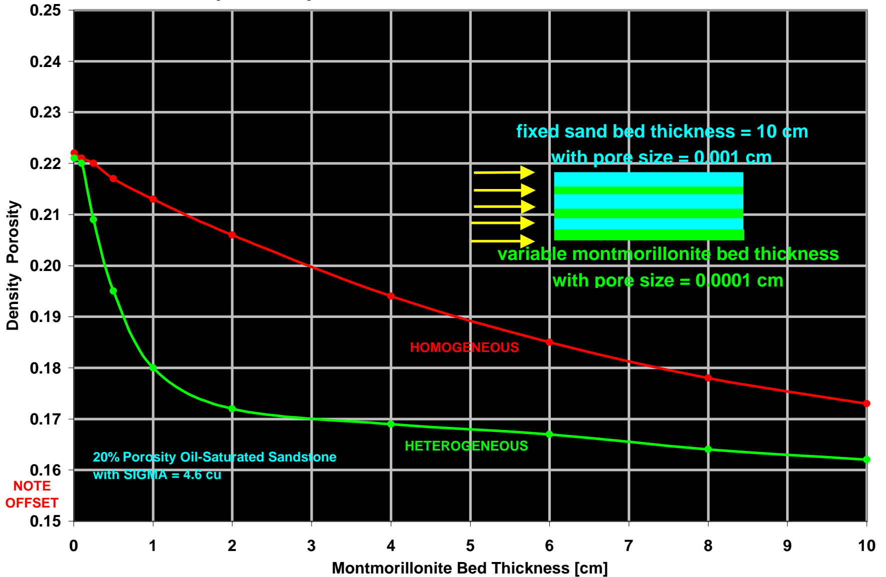
Density Porosity versus Montmorillonite Bed Thickness
