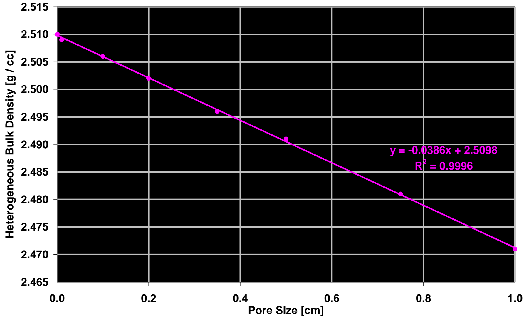
Heterogeneous Bulk Density versus Pore Size for a 20% Porosity Oil-Saturated Dolomite
