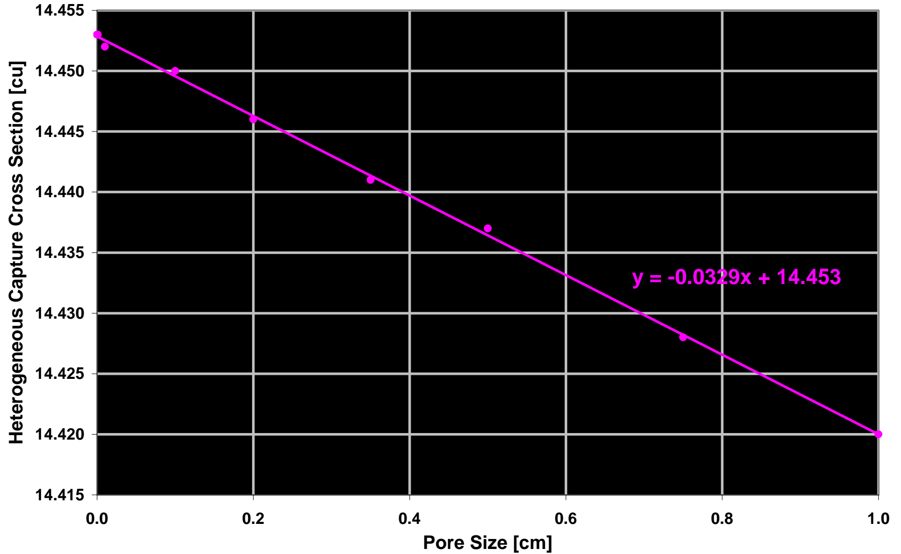
Heterogeneous Capture Cross Section versus Pore Size for a 20% Oil Saturated Dolomite
