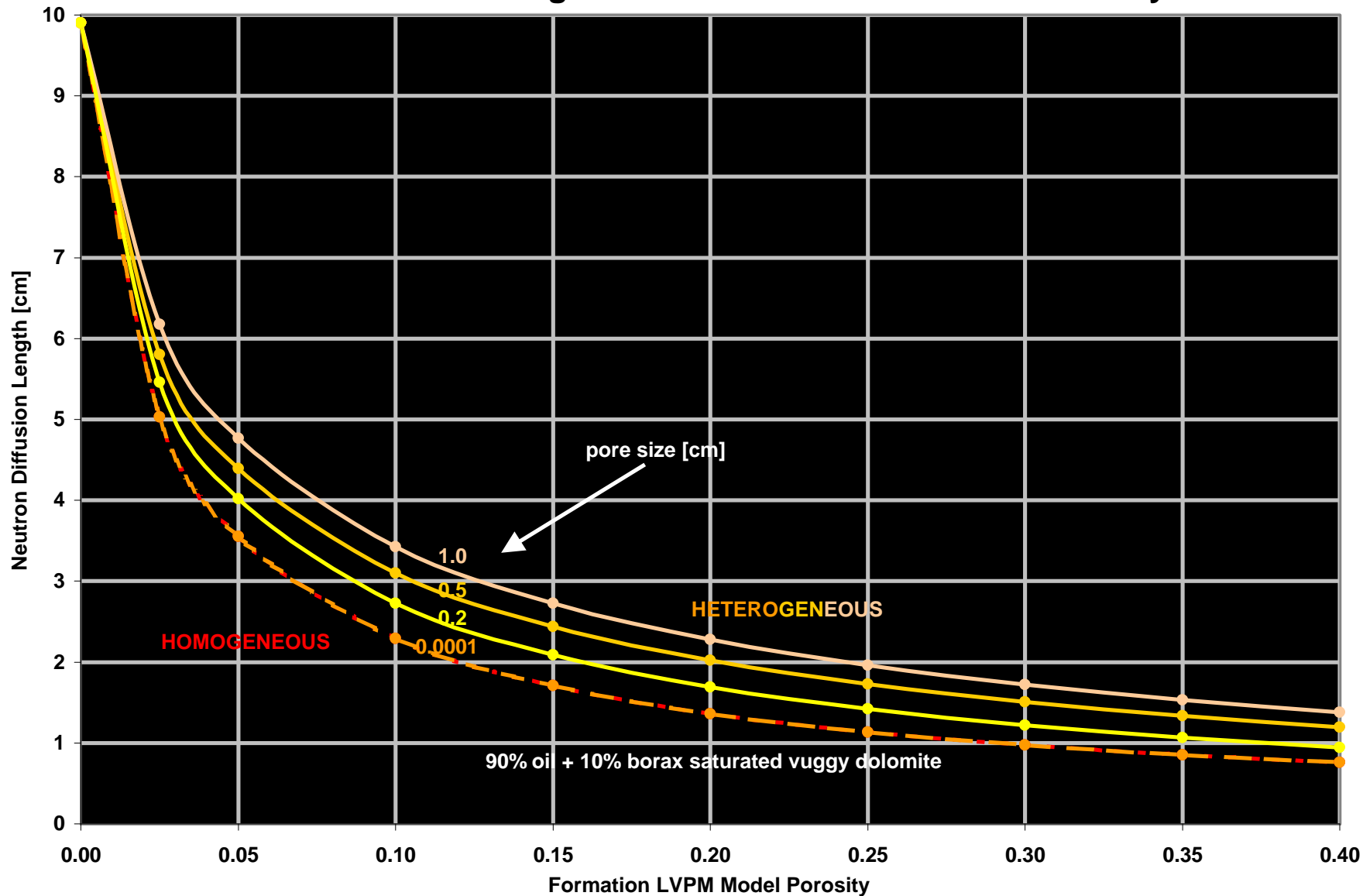
Neutron Diffusion Length vs Formation LVPM Model Porosity
