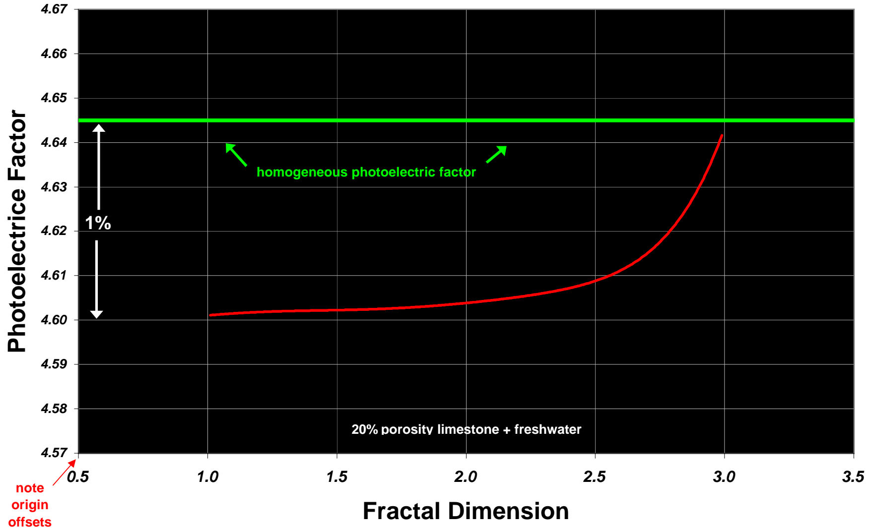
Apparent Photoelectric Factor versus Fractal Dimension with a Constant True Porosity of 0.20
