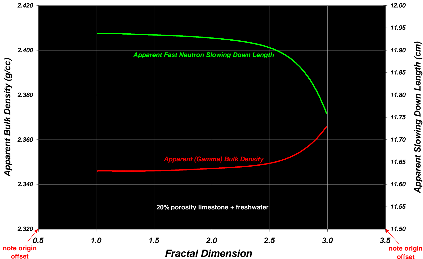
Apparent Bulk Density & Apparent Slowing Down Length versus Fractal Dimension with a Constant True Porosity of 0.20
